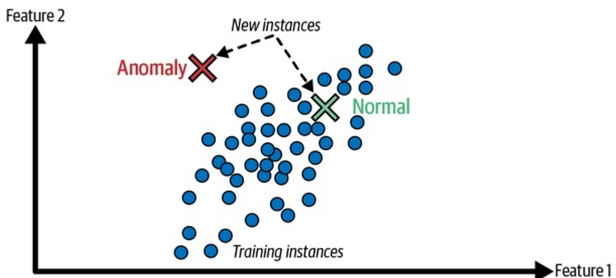
Figure 1-10. Anomaly detection
