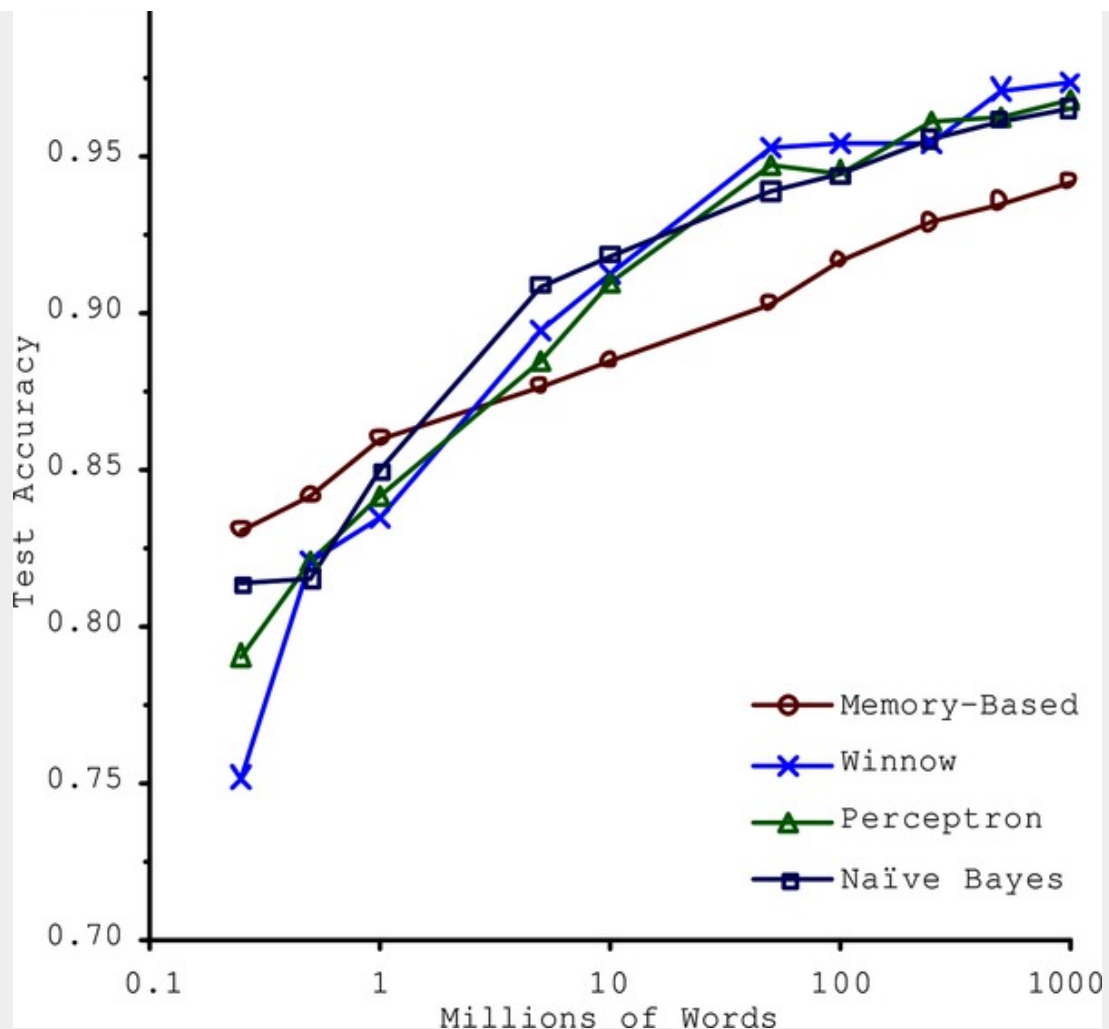
Figure 1-21. The importance of data versus algorithms 8
