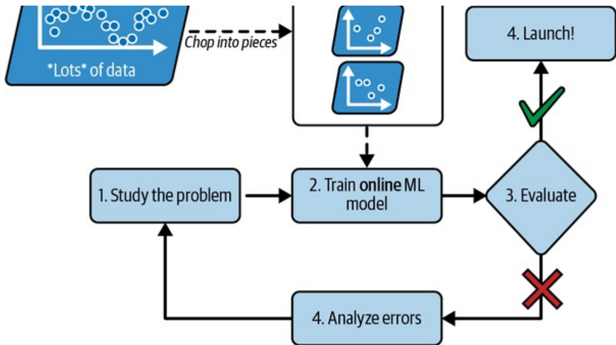
Figure 1-15. Using online learning to handle huge datasets
