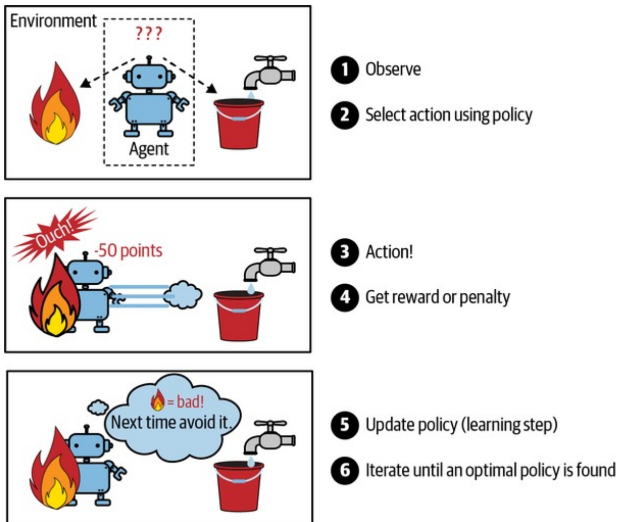
Figure 1-13. Reinforcement learning
