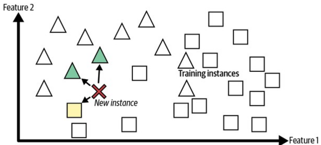
Figure 1-16. Instance-based learning
